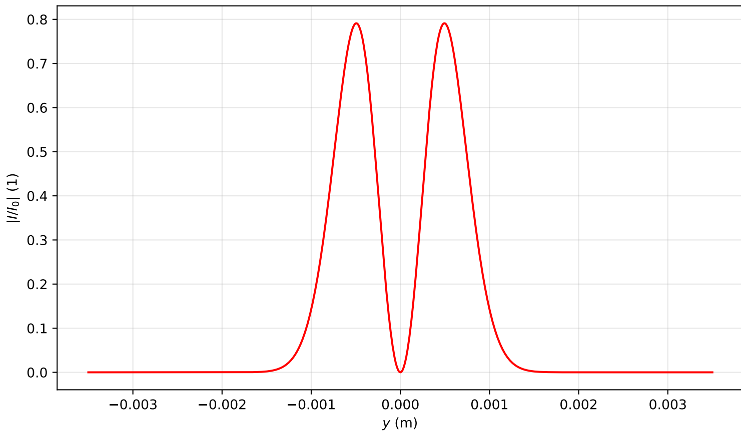
Intensity profile I(x=0, y, z=0.080)/I_0 , P_{in}=5.0P_{cr} , artificial time
